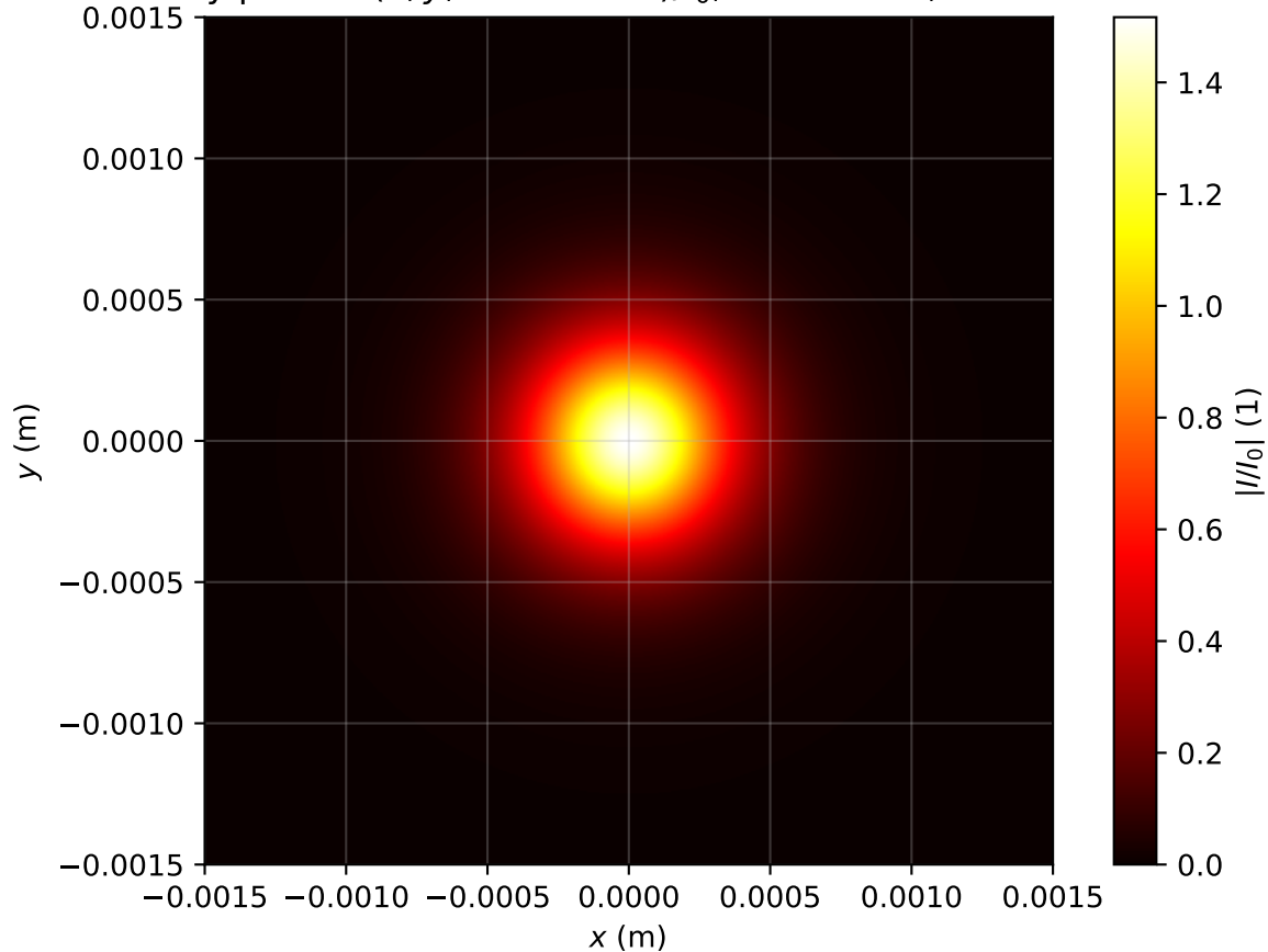
Intensity profile I(x, y, z = 3.344m)/I_0 , \text{Pin}=0.9\text{Pcr} , artificial time
